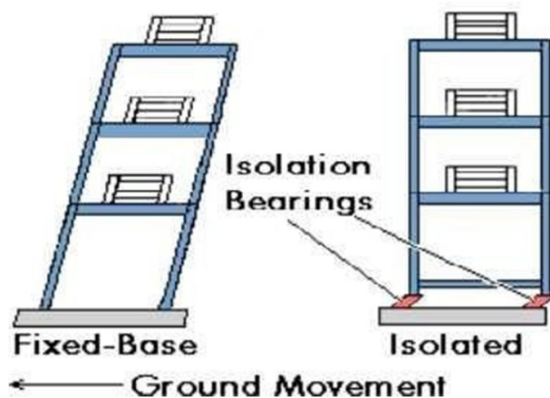
Figure 1: Typical explanation of base isolation system
