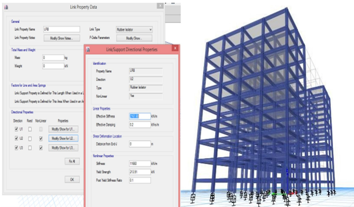
Figure 5: Building after the incorporation of LRBs at the base of it
