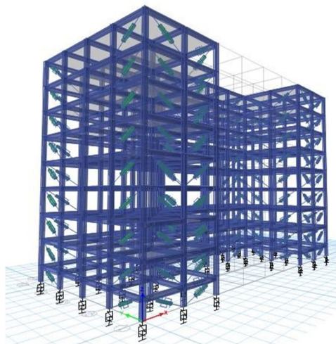
Figure 7: Building with the inclusion of LRB and Friction Dampers
