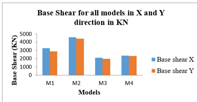
Figure 9: Base Shear of all the models in both X and Y direction
