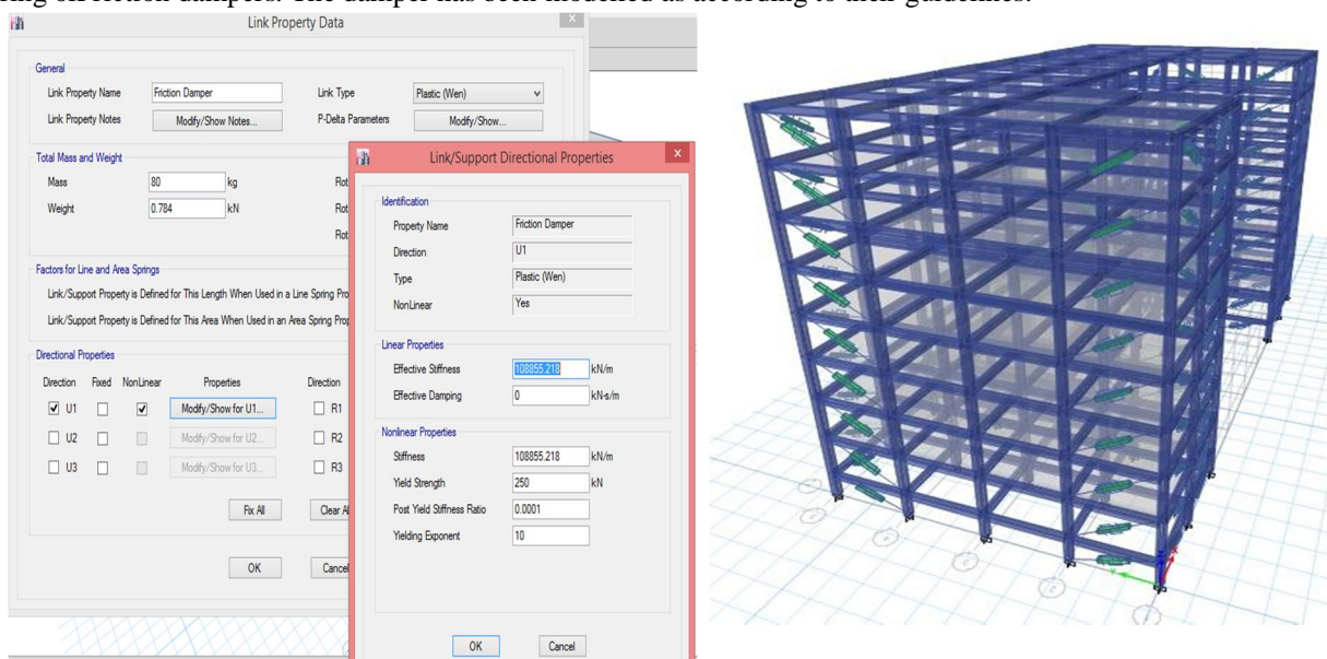
Figure 6: Building after the incorporation of Friction Dampers
