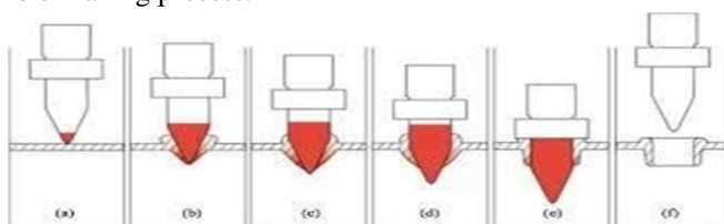
Fig -1: Process of Friction Drilling
