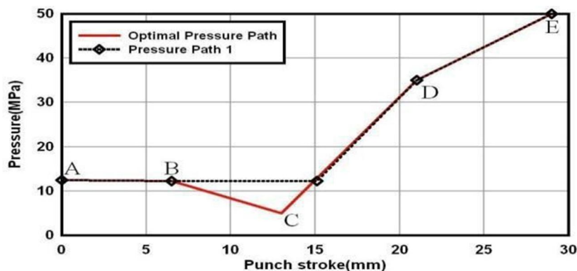
Fig 8.(a) Pressure path 1(27)
