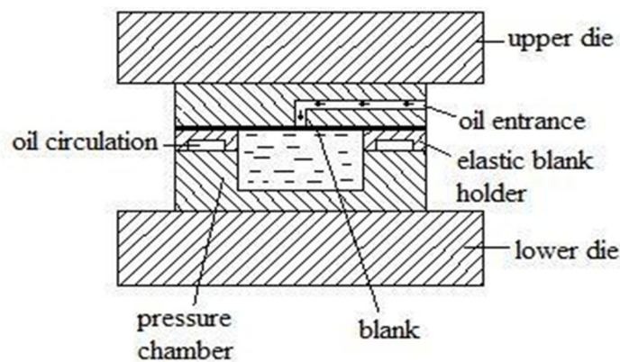
Fig.4 A simplified schematic of tool set-up for active-elastic blank holder system (1)
