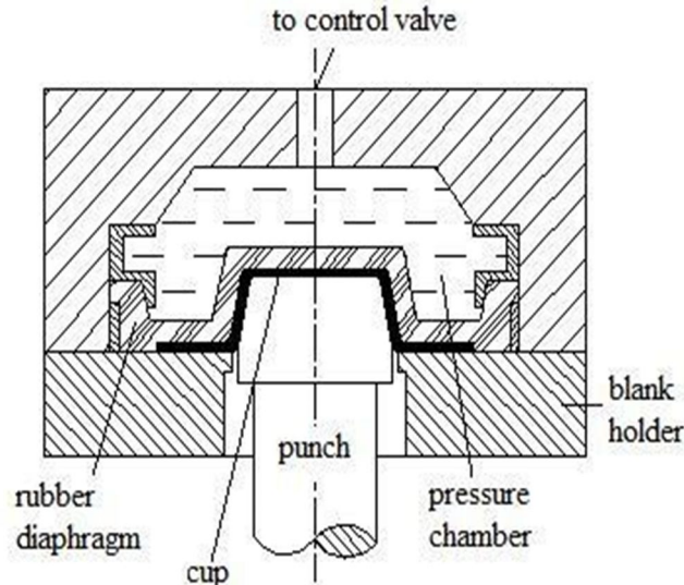
Fig.2 Tool set-up for standard hydroforming (17)
