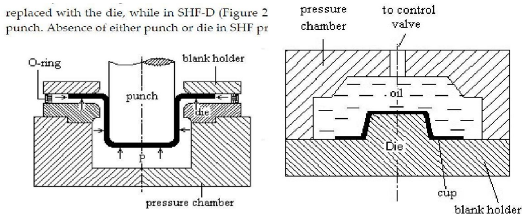
Fig. 1. Schematic of the sheet hydroforming process: (a) SHF-P, (b) SHF-D [17]
