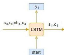
Figure 11: Timestep t=1
