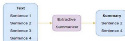
Figure 1: Extractive Summarization
