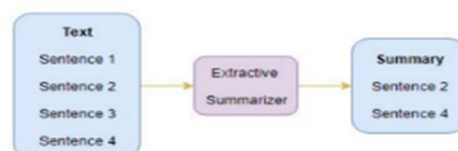
Figure 1: Extractive Summarization
