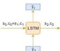
Figure 12: Timestep t=2
