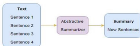
Figure 2: Abstractive Summarization
