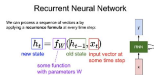
Figure 8: Basic Equations of RNN
