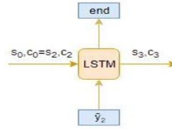
Figure 13: timestep t=3
