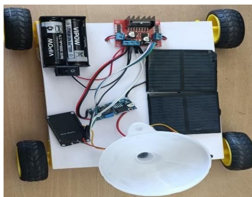
Fig. 2. Fabricated prototype of the solar-powered Bluetooth-controlled agricultural seed sowing robot.
