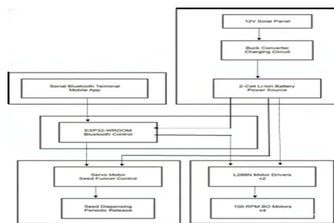
Fig. 1. Block diagram of the proposed solar-powered Bluetooth-controlled seed sowing robot.
