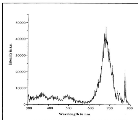
Figure 2 (b) Synchronous luminescence spectrum of leaf of Ficus benghalensis [family-Moraceae].
