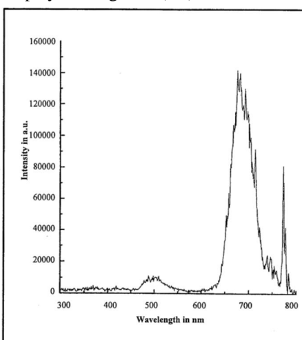
Figure 2 (a) Synchronous luminescence spectra of plants of Ficus religiosa [Family-Moraceae].
