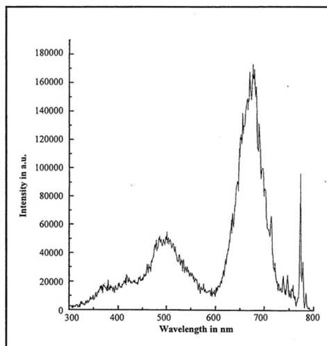
Figure 2 © Synchronous luminescence spectrum of leaf of Hibiscus rosasinensis [Family-Malvaceae].
