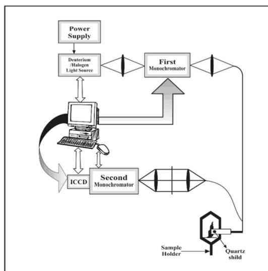
Figure 1 Experimental arrangement for recording synchronous luminescence spectra of plants leaves.
