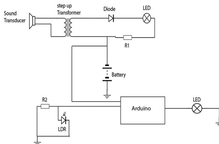
Fig 2: Circuit Diagram
