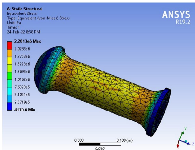
Stress Analysis
