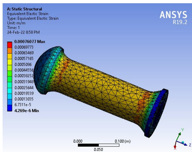
Strain Analysis
