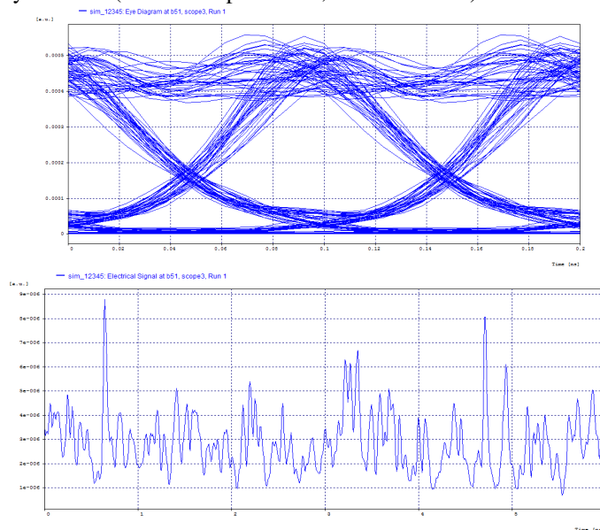
Graph of Electrical Signal And Eye Pattern (for D = 16 ps/nm/km, \alpha = 0.2 dB/km):
