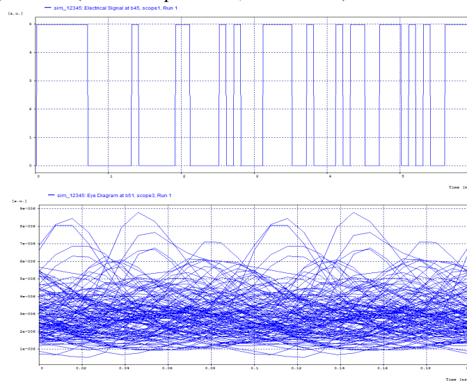
Graph of Electrical Signal And Eye Pattern (for D = 16 ps/nm/km, \alpha = 0.5 dB/km):
