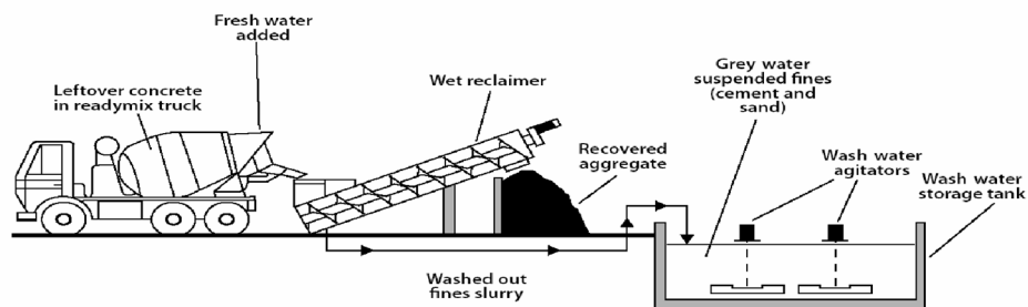
Figure2: Typical system for recycling wash water/aggregate recovery
