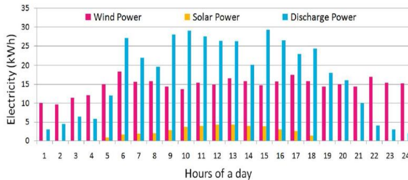
Fig. 5. Hourly generated electricity by both wind and solar from the proposed method.
