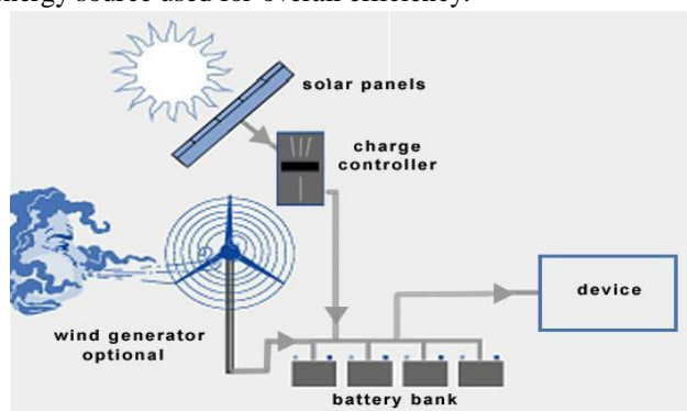
Fig. 1 Schematic of a conventional photovoltaic Hybrid System.
