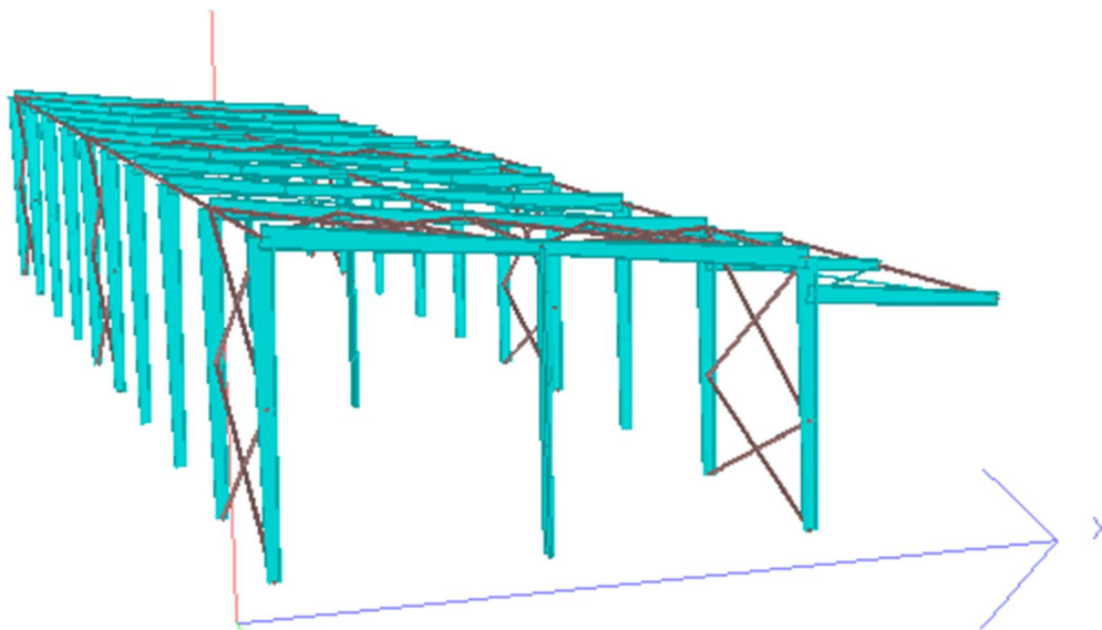
Figure 2 – 3D view
