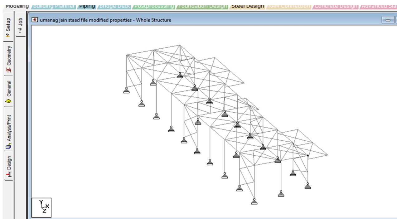
Figure 1 – Isometric view
