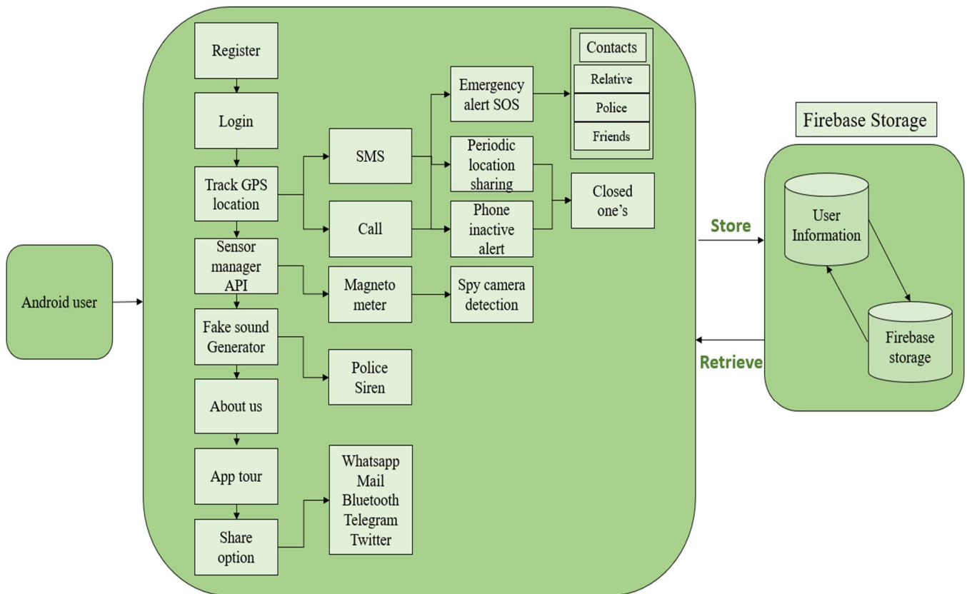
Figure.4: Architecture Diagram
