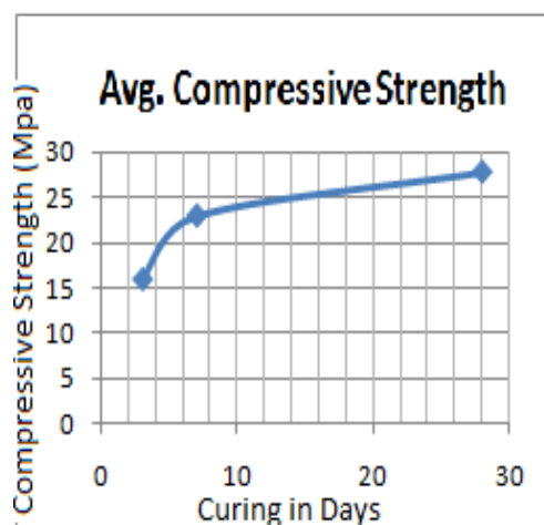
FIG. 3 COMPRESSIVE STRENGTH TEST RESULTS OF ECO FRIENDLY CONCRETE (STEAM CURING)
