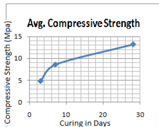
Fig. 2 Compressive Strength Test Results of Eco Friendly Concrete (Water Submerged Curing)
