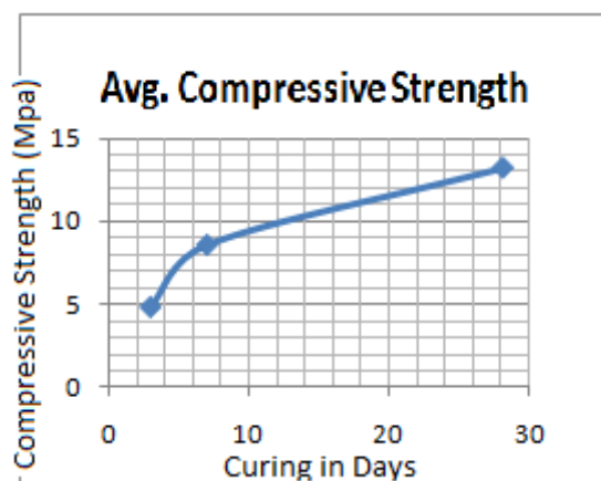
Fig. 2 Compressive Strength Test Results of Eco Friendly Concrete (Water Submerged Curing)
