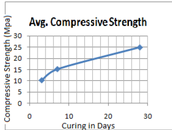
Fig. 1 Compressive Strength Test Results Of Ordinary Concrete
