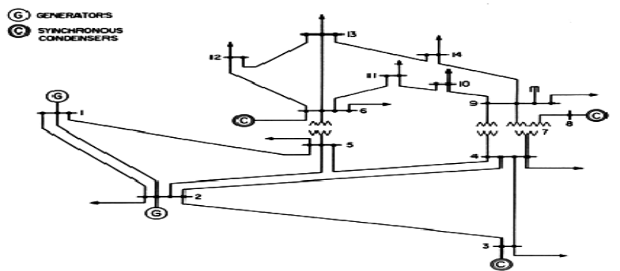
Fig1: IEEE-14 bus system
