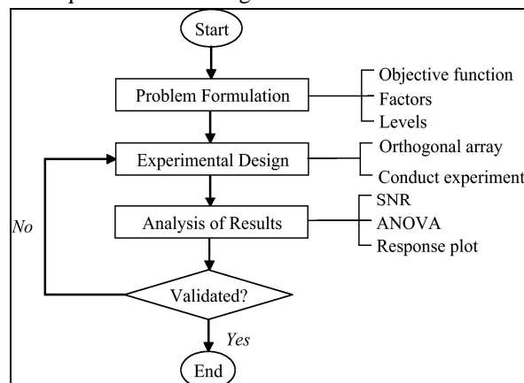
Figure 2 Taguchi Technique
