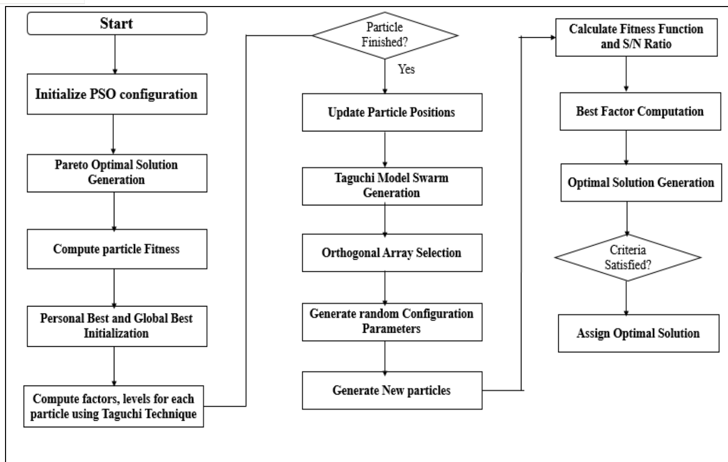
Figure 4Taguchi and PSO implementation without optimal solution
