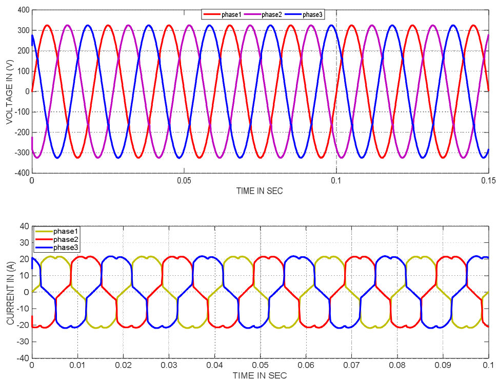
Fig. 6 Voltage and Current Waveform with Double Tuned Harmonic Filters.
