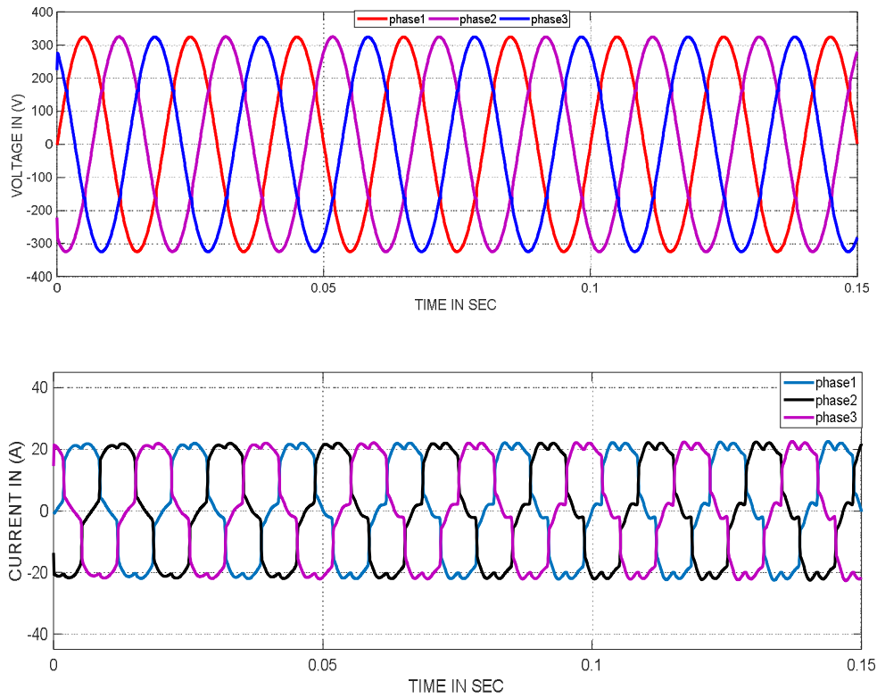
Fig. 4 Voltage and Current Waveform with Single Tuned Harmonic Filters.
