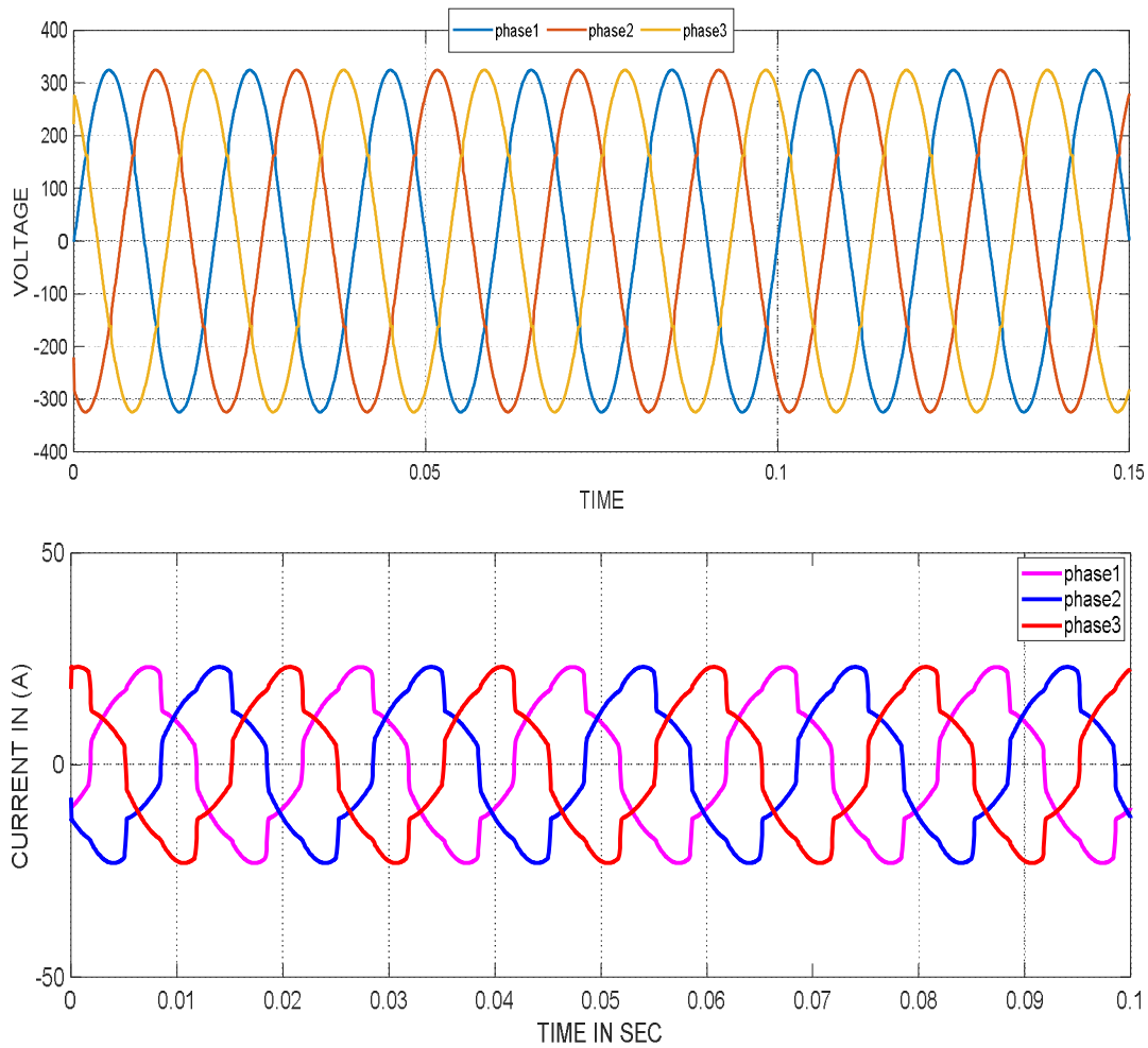
Fig. 2 Voltage and Current Waveform without Filters
