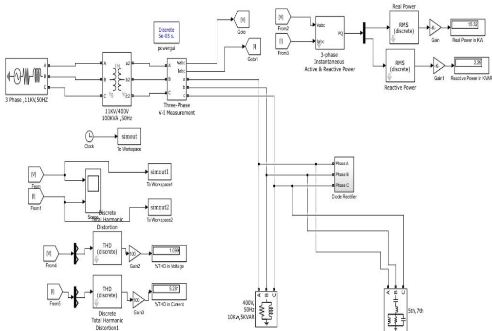
Fig. 5 MATLAB based model with three-phase Double tuned passive Filters.
