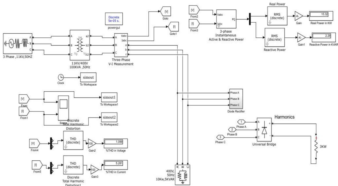
Fig. 1 MATLAB based model without Passive Filters.
