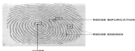
Fig.1. Fingerprint Image
