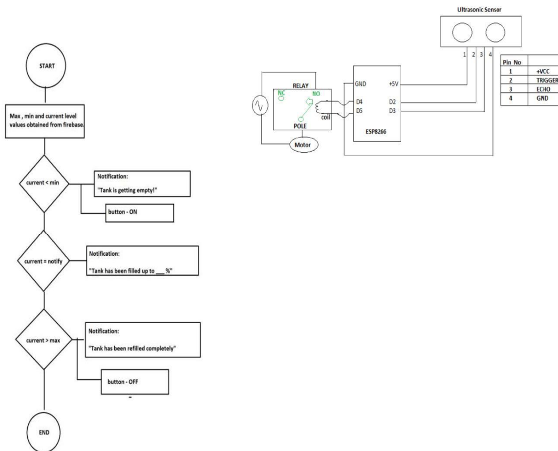
Fig 6. Water level management block
