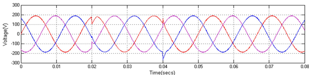
Fig. 8(c) Load voltage.
