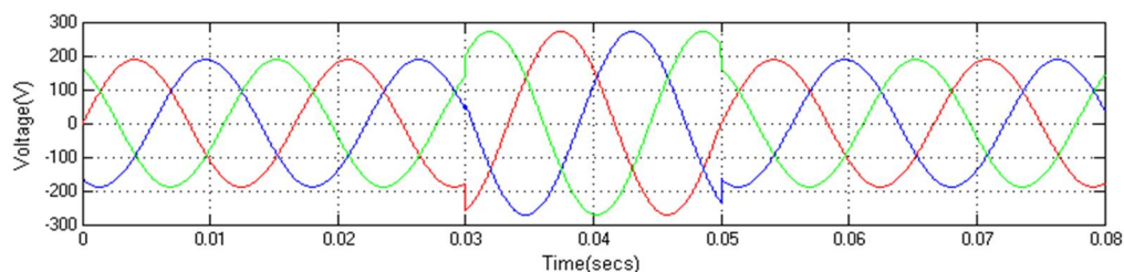
Fig. 7 (a) Performance of DVR during Voltage swell.
