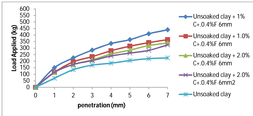
Figure 3 CBR value of Clayey Sub-grade Soil mixed with Cement 0.4% Recron Fiber (6mm)under Un-soaked condition
