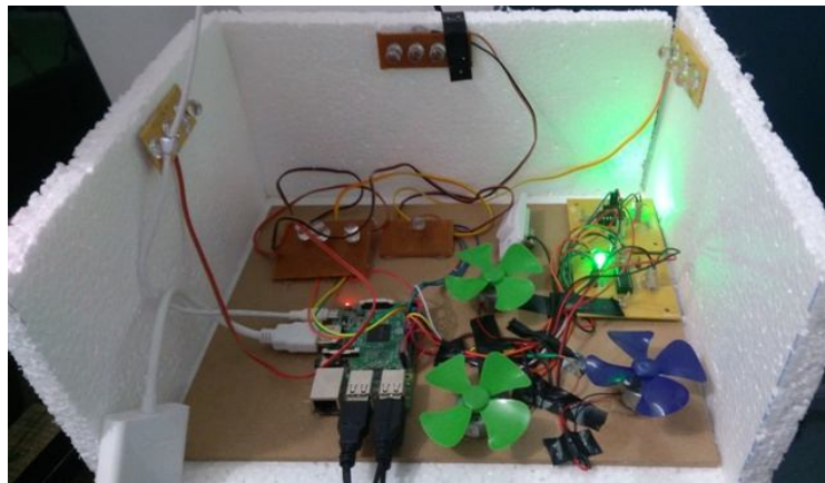
Figure 2: experimental setup
