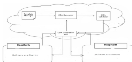
Fig. 1. CDA generation system
