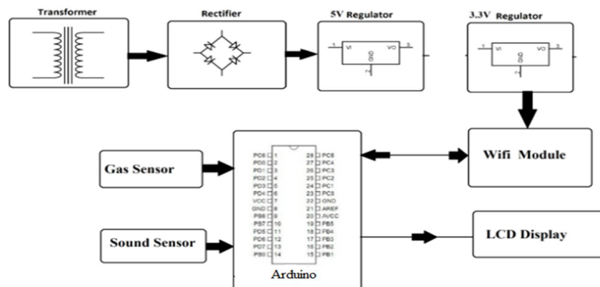
Fig. 2: Block Diagram
