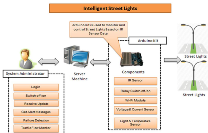
Figure: - System Architecture of Intelligent Street Lights System.
