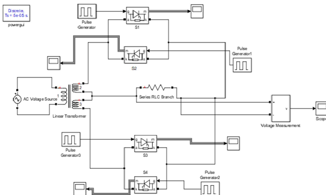
Fig 1: Simulation Circuit For CYCLO-Convertor With R Load
