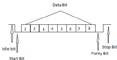
Fig 2. UART FRAME FORMAT
