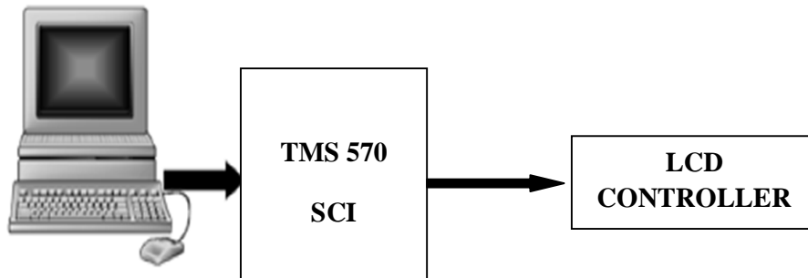
Fig. 3 Application design of UART
