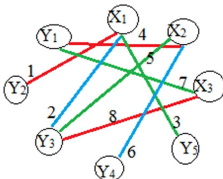
Fig 5. Bipartite graph
