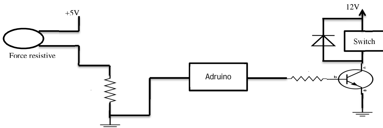
Figure 1: Block Diagram of Proposed System
