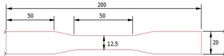
Fig – 3: Standard tensile test specimen ASTM E8
