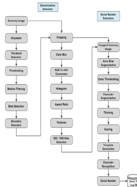
Fig 1. System Workflow [1]
