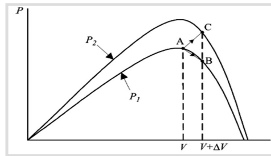
Fig. Divergence of P&O from MPP
