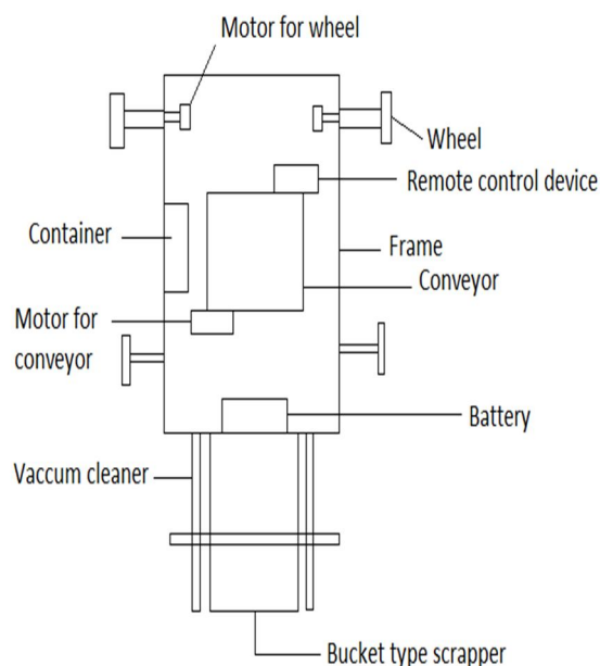
Design of scrap collecting vehicle
