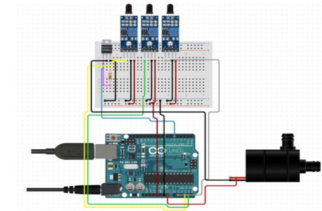
Fig. 3 Arduino UNO, three Flame Sensors & Water Pump Connection
