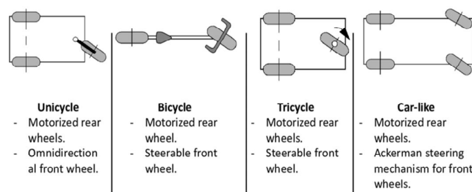
Fig. 1 Types of steering mechanisms
