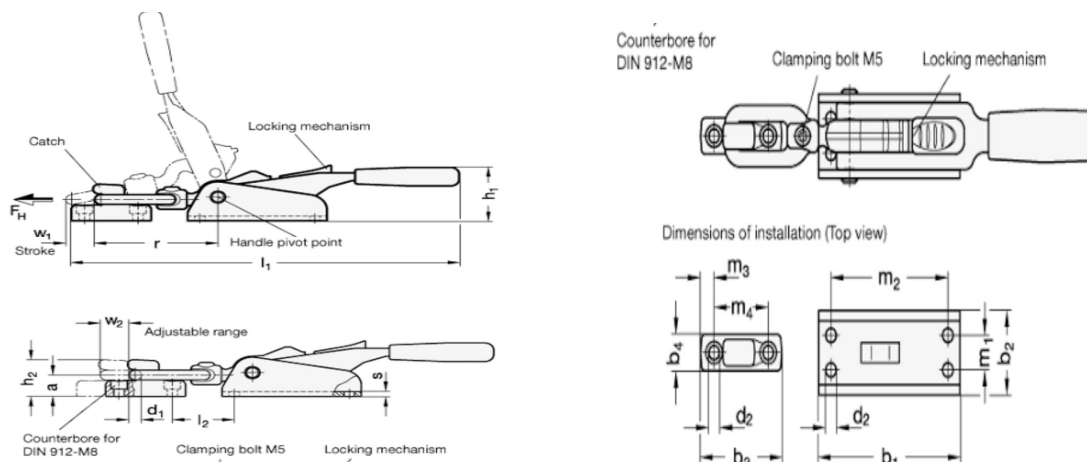
Fig. 2 Latch mechanisms
