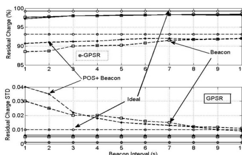
Figure 2: Average (upper plot) and standard deviation (lower plot) of the residual charge of network nodes.
