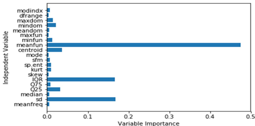
Figure 2. Importance of individual feature in the model.
