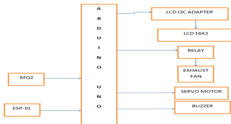
Fig1.Block diagram of Gas Monitoring system using Arduino
