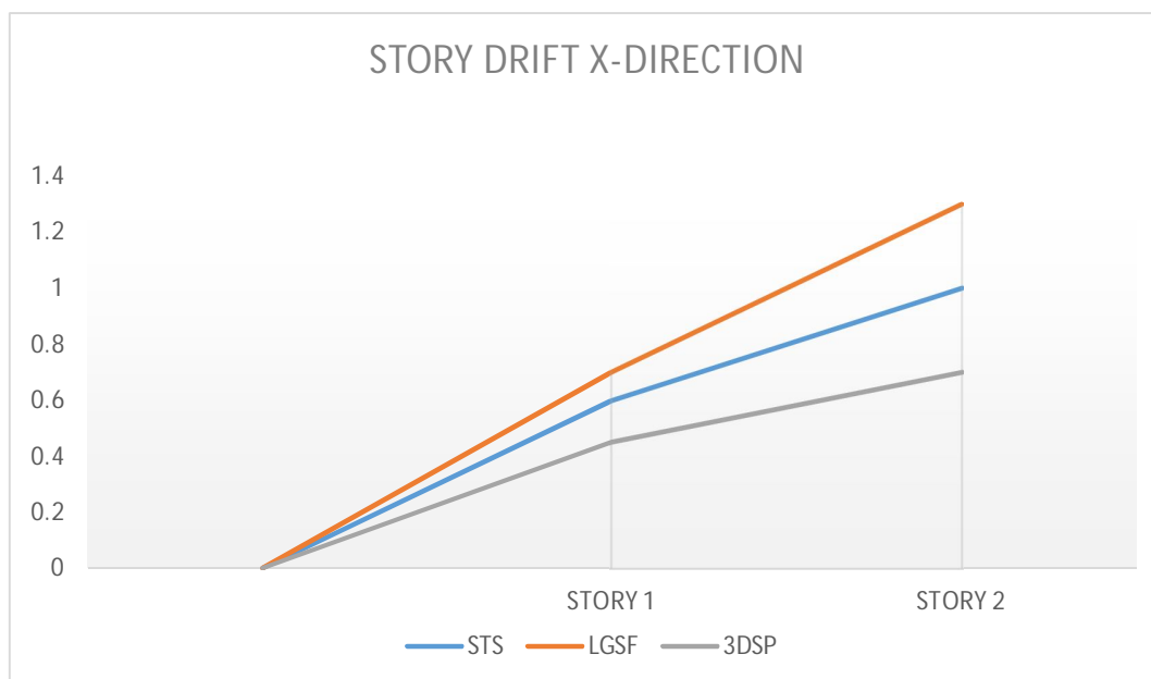
Chart2:- Story Drift in X-direction
