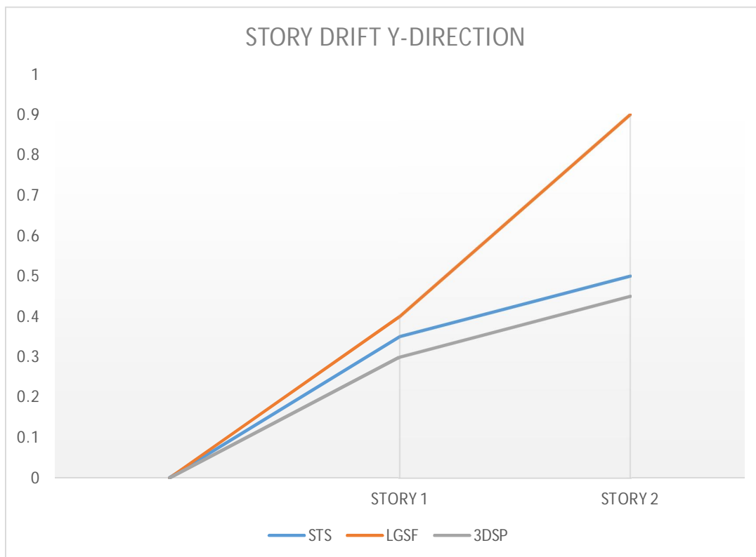
Chart3:-Story Drift in Y-direction
