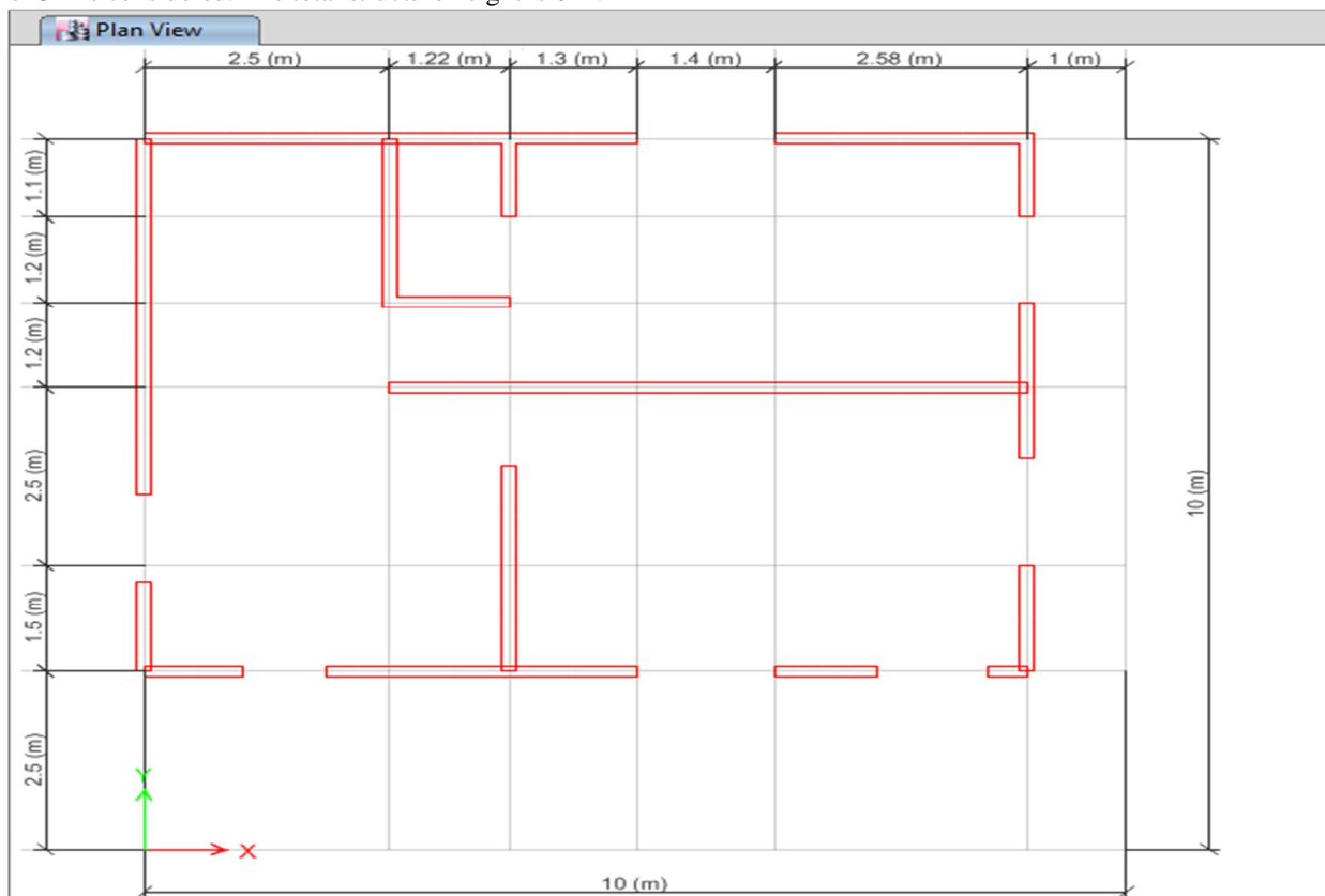
Fig-1:-Dimensions of ground floor plan in Example Building- Units in m
