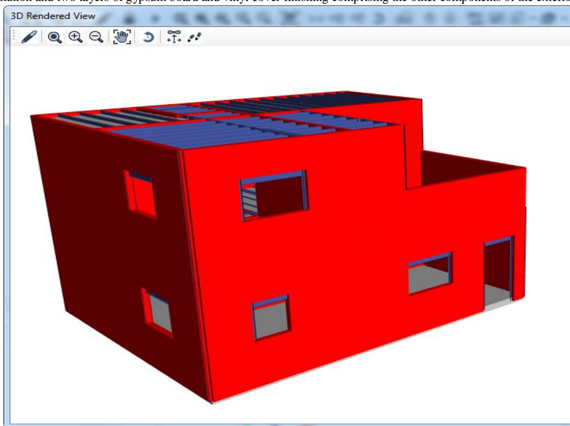
Fig3:-3D modeling of light gauge steel structure in ETABS.
