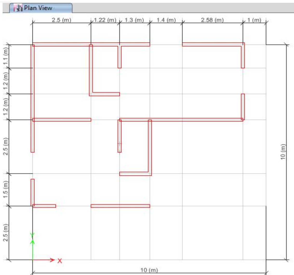
Fig2:-Dimensions of first floor plan in Example Building- Units in m
