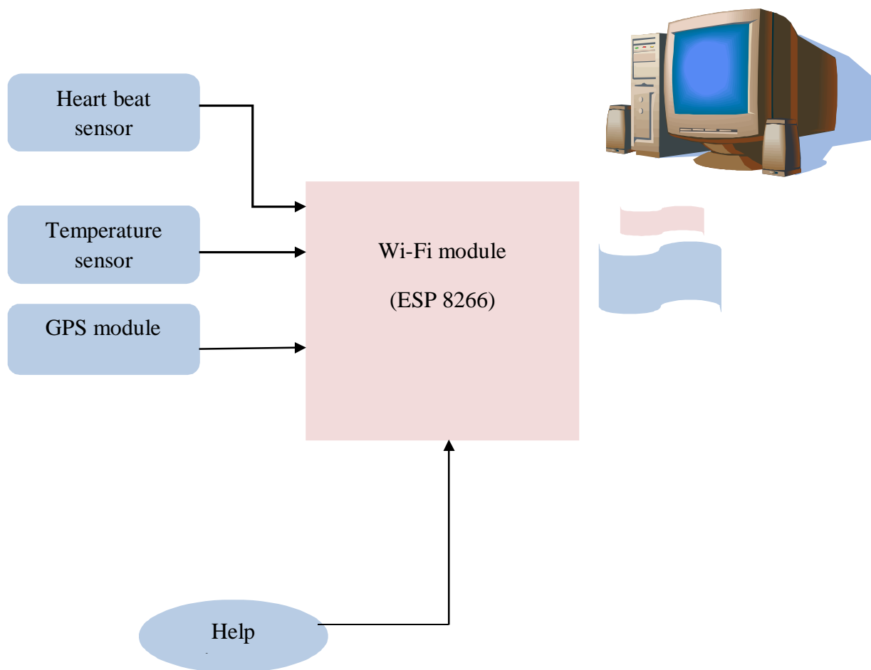
Fig(5.1): Block diagram of soldier unit
