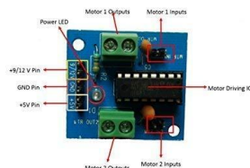
Fig.5 motor driver
