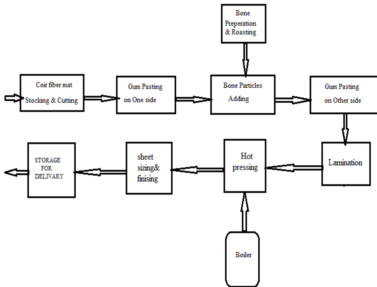
Fig. 2 Process diagram
