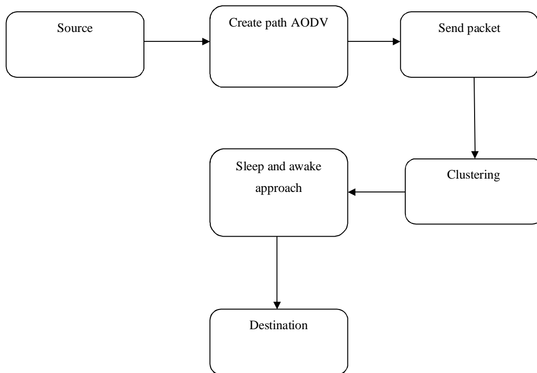
Figure 1: System architecture
