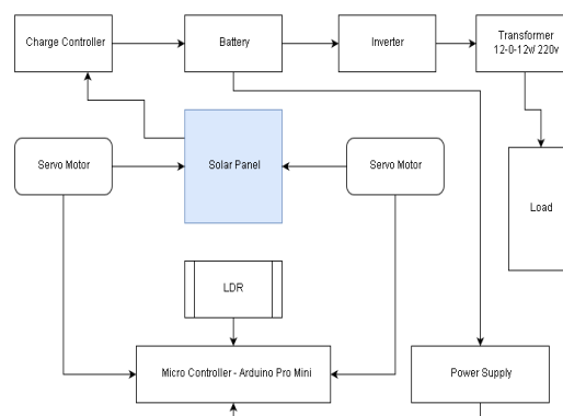
Fig 1.1: Block Diagram.
