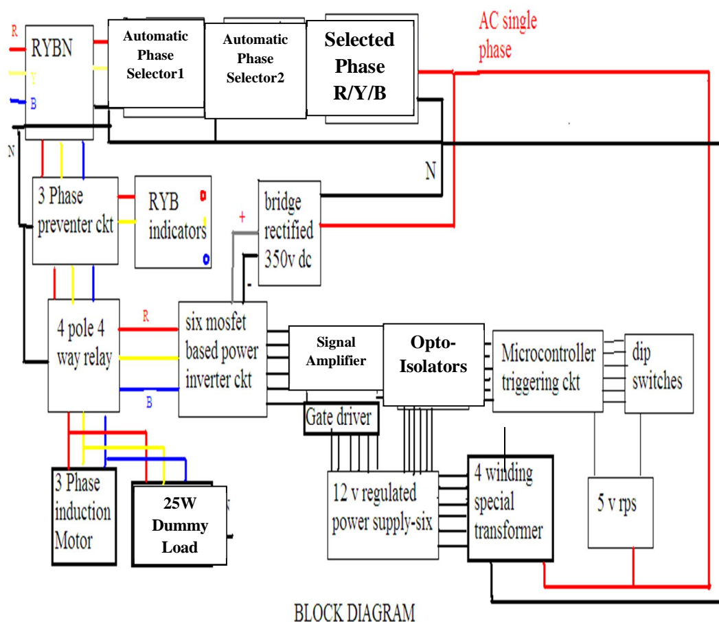
Fig.1. Block Diagram
