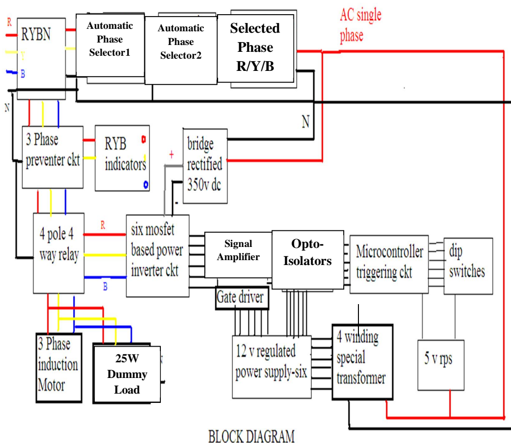
Fig.1. Block Diagram
