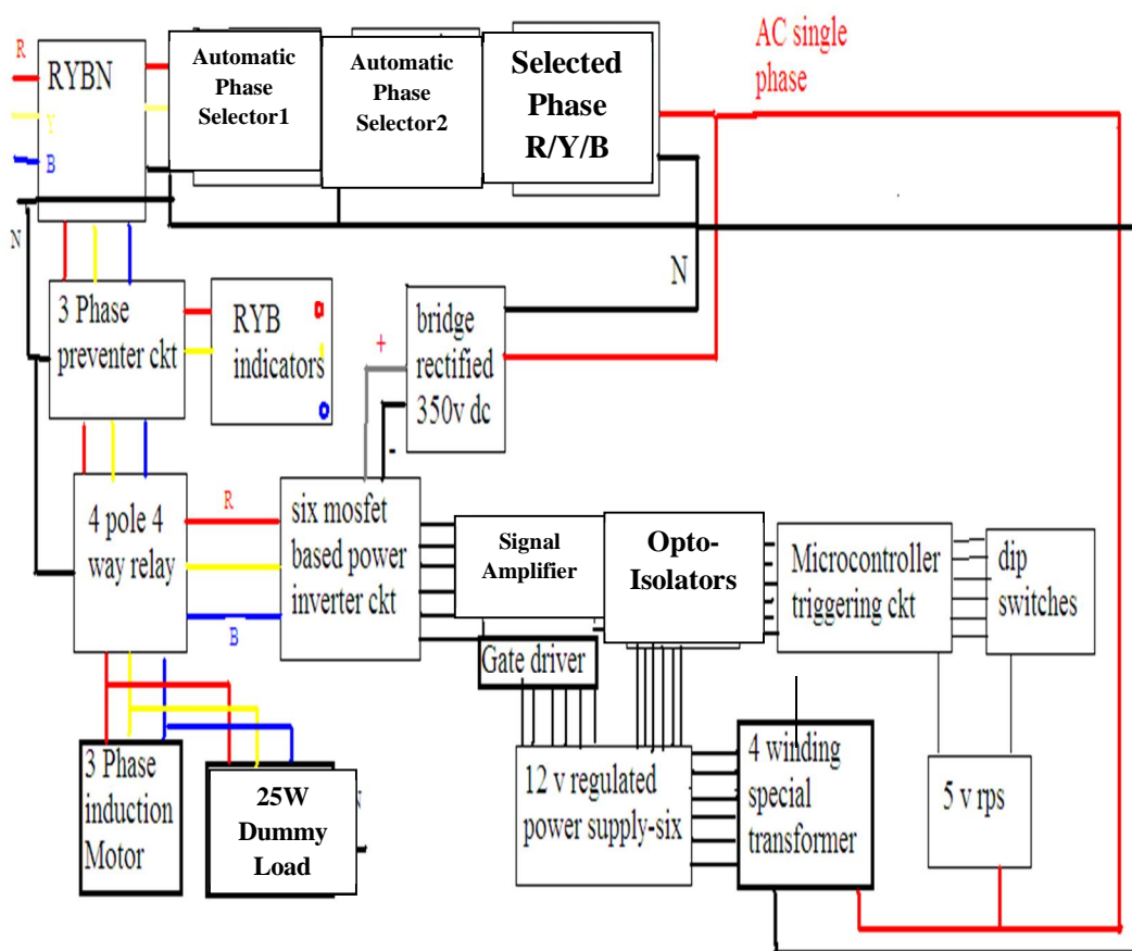
BLOCK DIAGRAM
