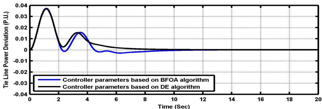
Fig. 12: Tie Line Power Deviation for 5% Step Load Change in Area-2 at \alpha=\pm 0.025
