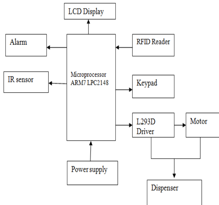
Fig 2: Block diagram of all time medicine counter
