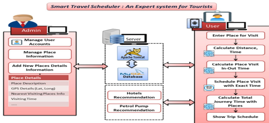
Figure 1: System Architecture
