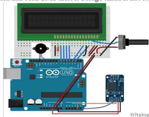
Connection Diagram
