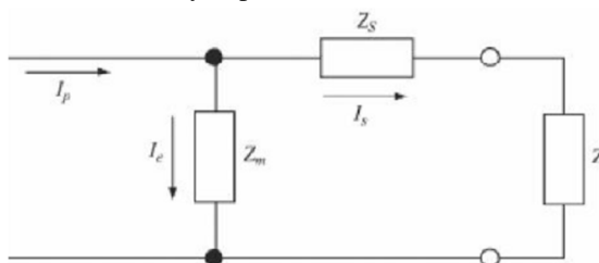
Fig. 1 – Equivalent Electric Circuit of a Current Transformer
